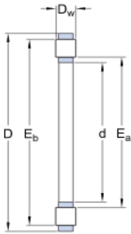
Cylindrical Roller Thrust Bearing
